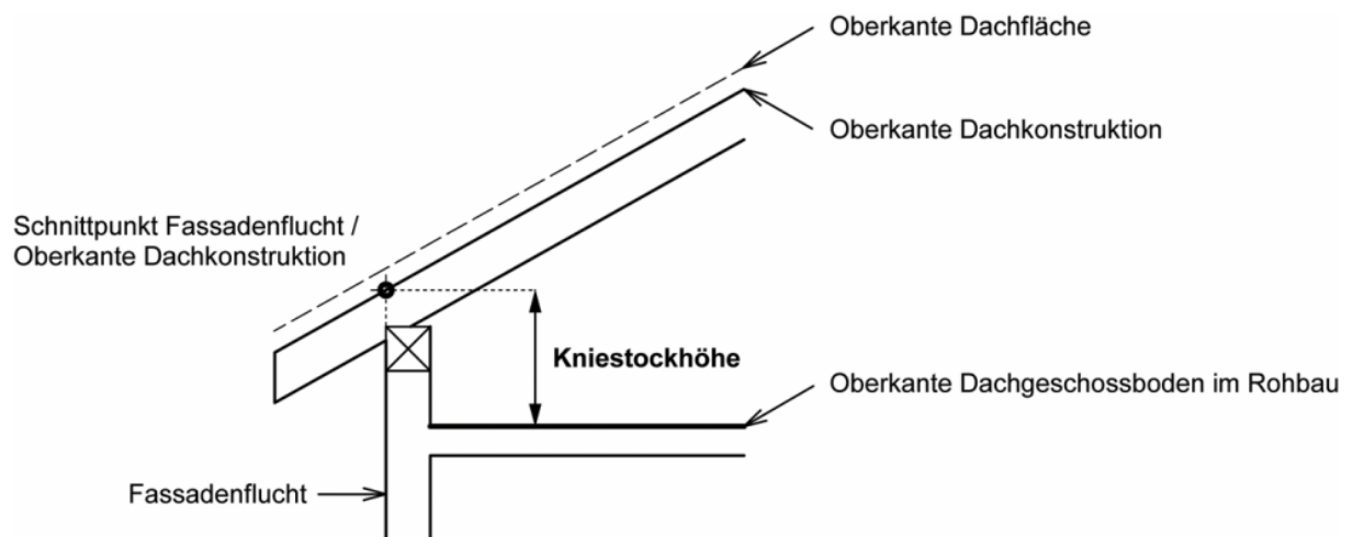
Figur 5.3 Kniestock
