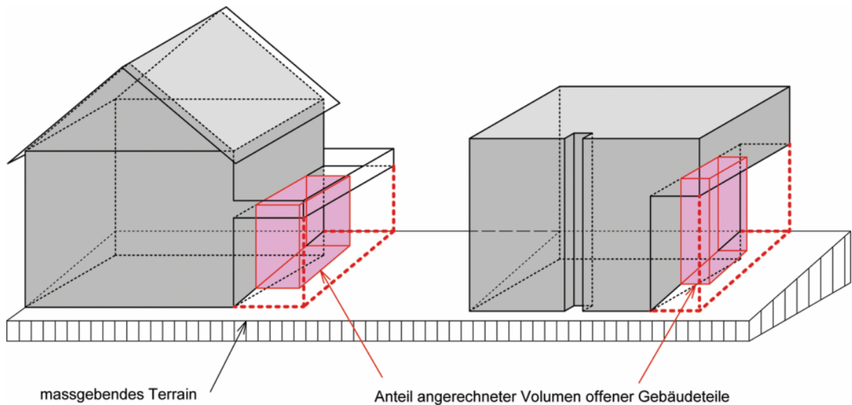
Figur 8.3 Baumassenziffer
